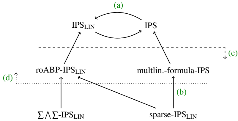
Figure 1: This diagram summarizes the main results of this paper, listing some of the upper bounds given in Section 4, as well as some of the functional lower bounds of Section 5. The lower bounds via multiples (Section 7) are not included here, as those lower bounds are slightly non-standard. Arrows indicate efficient simulation of proof systems, where unlabelled arrows are straightforward. Labelled results are as follows. (a) The simulation of general IPS by linear-IPS is given by Theorem 4.4. (b) The simulation of sparse-IPS LIN (equivalent to the Nullstellensatz system) by multilinear-formula-IPS is given by Theorem 4.12. (c) The region below the dashed line consists of proof systems where we prove superpolynomial lower bounds (Theorem 5.15). (d) The region above the dotted line can efficiently refute the subset-sum axiom \sum_i x_i + 1 = 0 over \bar{x} \in \{0, 1\}^n (Corollary 4.14, Theorem 4.15). In contrast, Polynomial Calculus cannot efficiently refute this system of equations ([41]).
